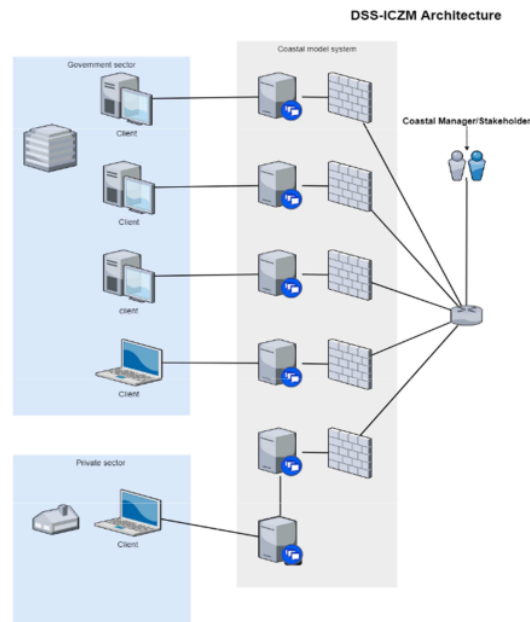
Fig. 1 DSS-ICZM architecture
