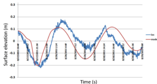
Fig. 4 Validation result between field (blue line) and model data (red line)
